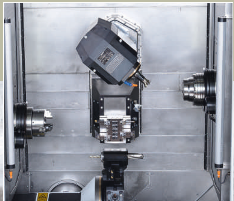
Version with subspindle and B-axis (LTBS-version)
